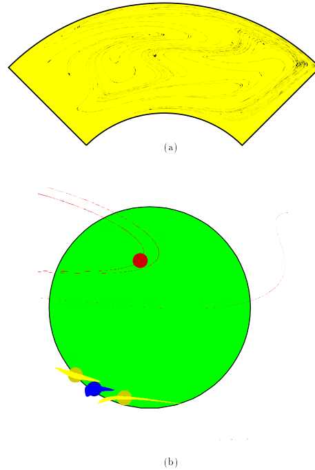
Figure 9. The elements of coherent structures: (a) part of unstable manifold of the hyperbolic point of period-1 in the centre of the initial blob; (b) deformation patterns of small circular blobs surrounding periodic points of higher orders
